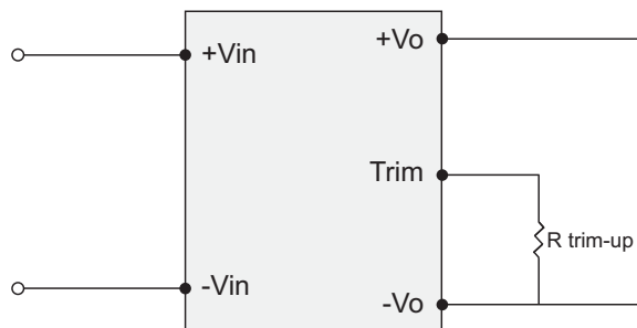
Trim-Up
