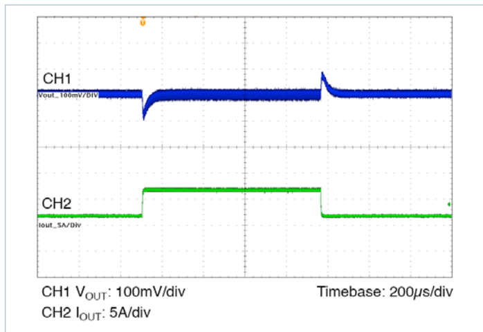
Figure 25 — Transient Response 2A to 7A, at 5A/µs
