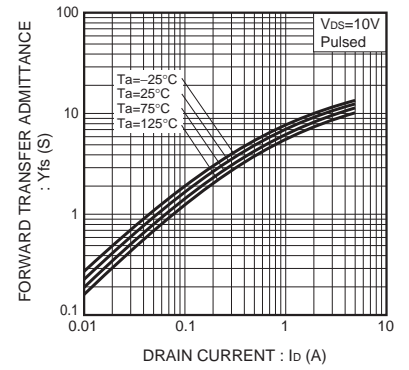
Fig.12 Forward Transfer Admittance vs. Drain current
