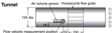
Figure 2: Wind Tunnel
